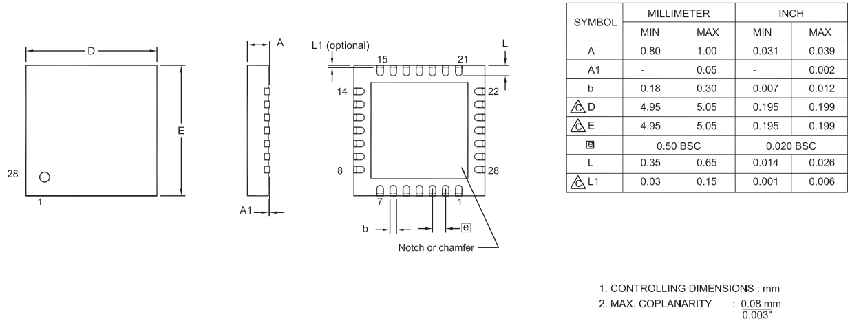
Figure 38. 28-Pin Quad Flat No-Lead (QFN) Package
